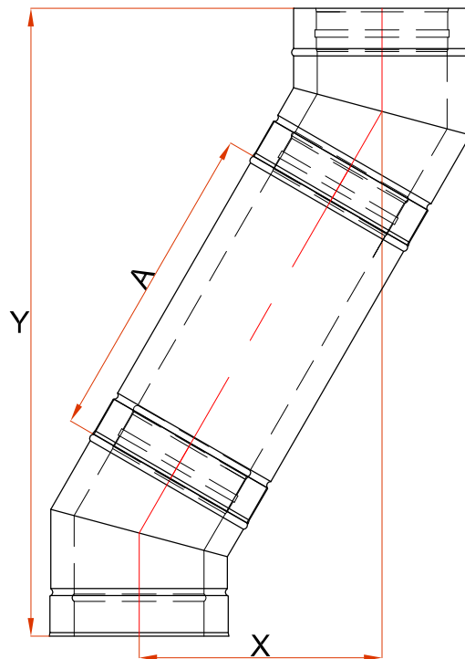
2 Coude 30°
